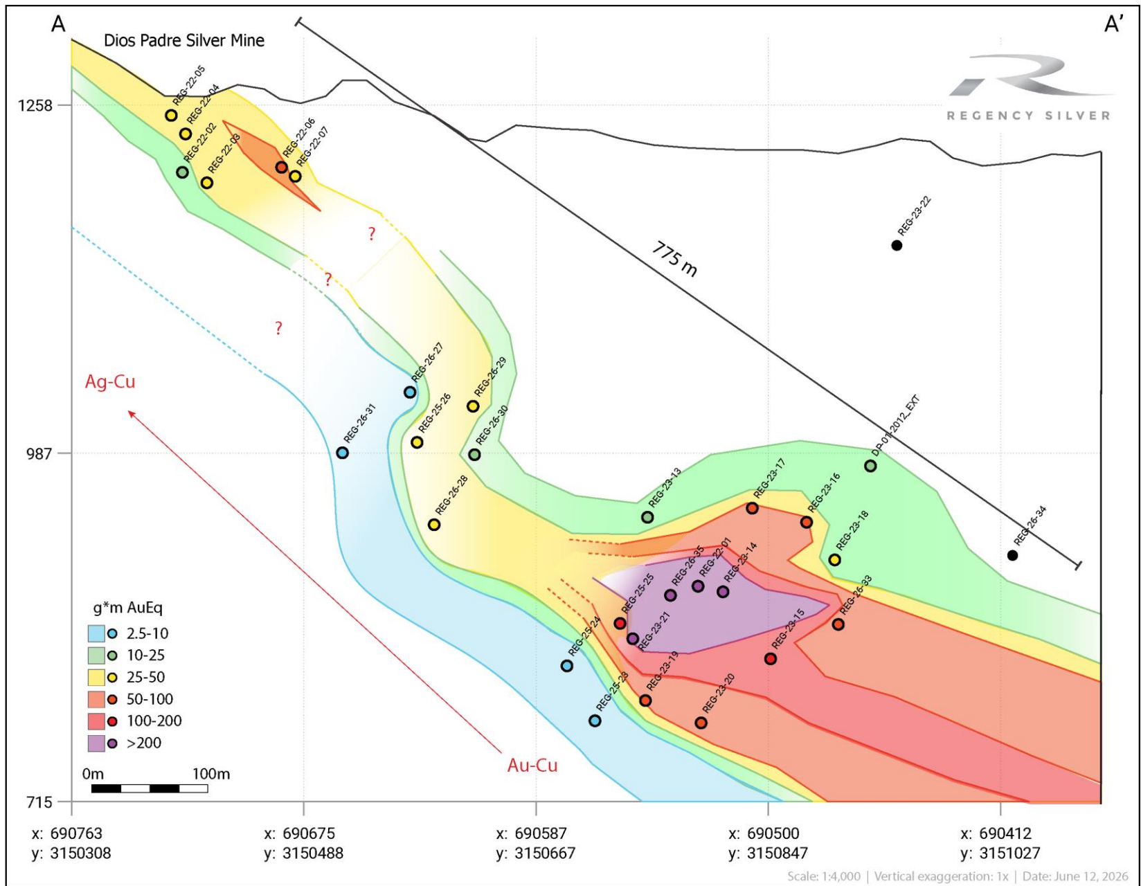
Figure 3: Long section for all holes in the Dios Padre breccia zone. Contours represent grade \times thickness (AuEq) for drill hole composites. AuEq is calculated for individual samples using $4250/oz Au, $65/oz Ag, and $6.25/lb Cu and 90% recoveries for each.
